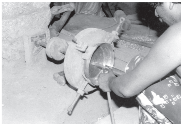
Fig. 13. Polishing of high-tin bronze vessel at Payangadi by hand lathe in 1991
